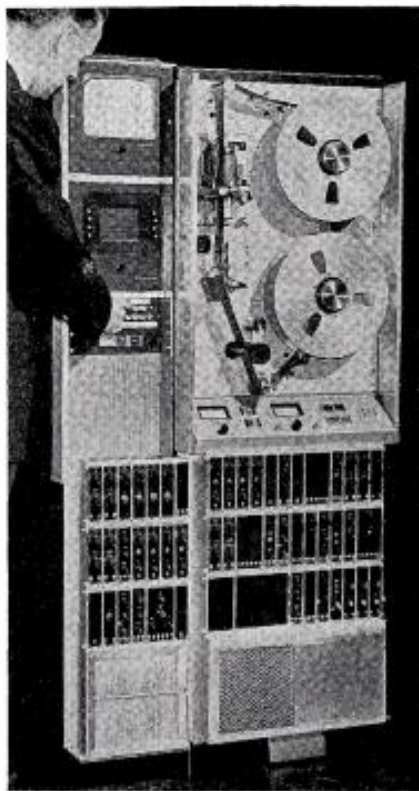
RCA's new compact TV tape recorder, the TR-4, showing vertical transport system and banks of plug-in circuit modules.
